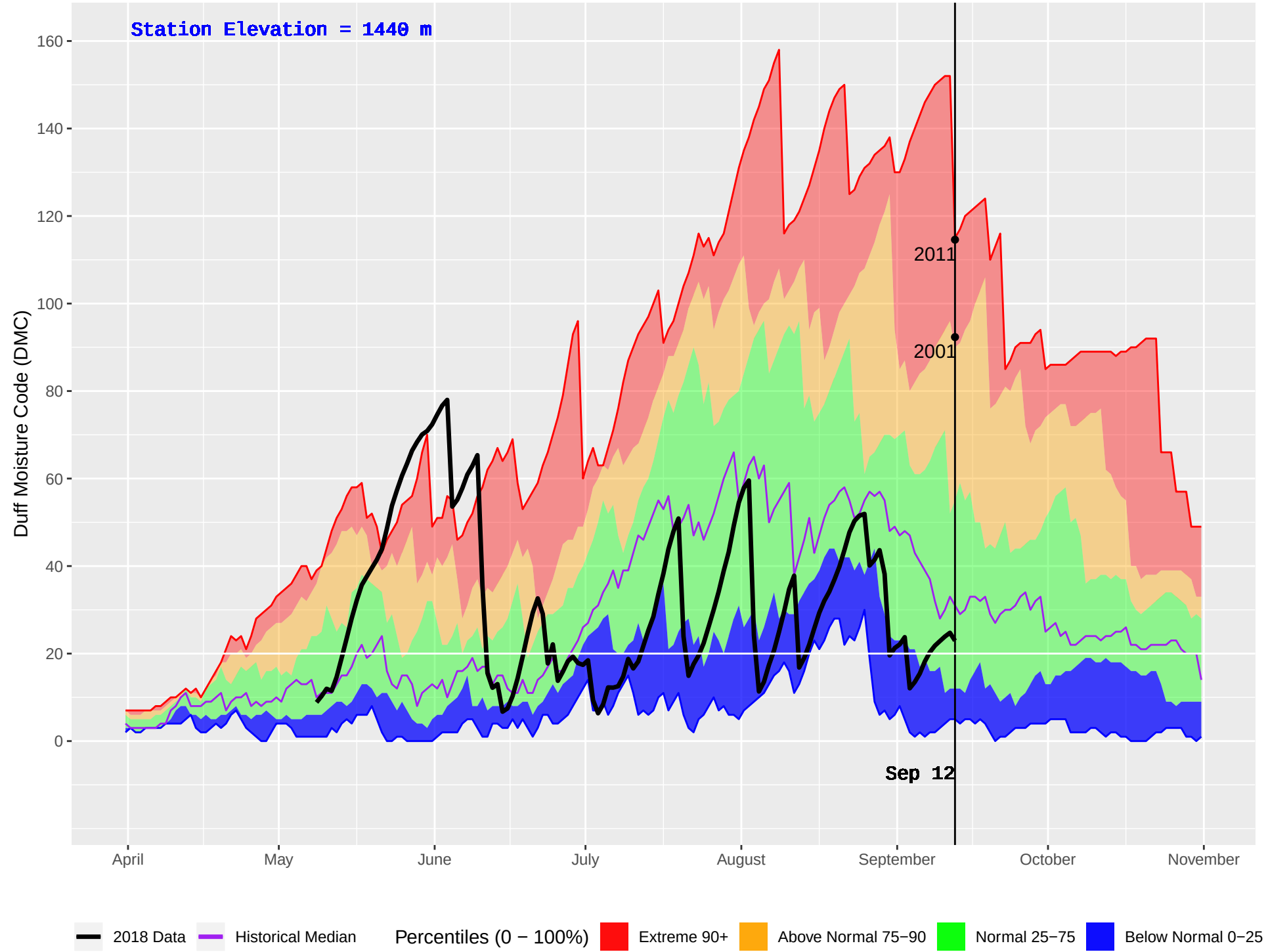
PASKA LAKE (326) : Historical (1999–2016) and Current (2018) Daily Duff Moisture Code (DMC)
