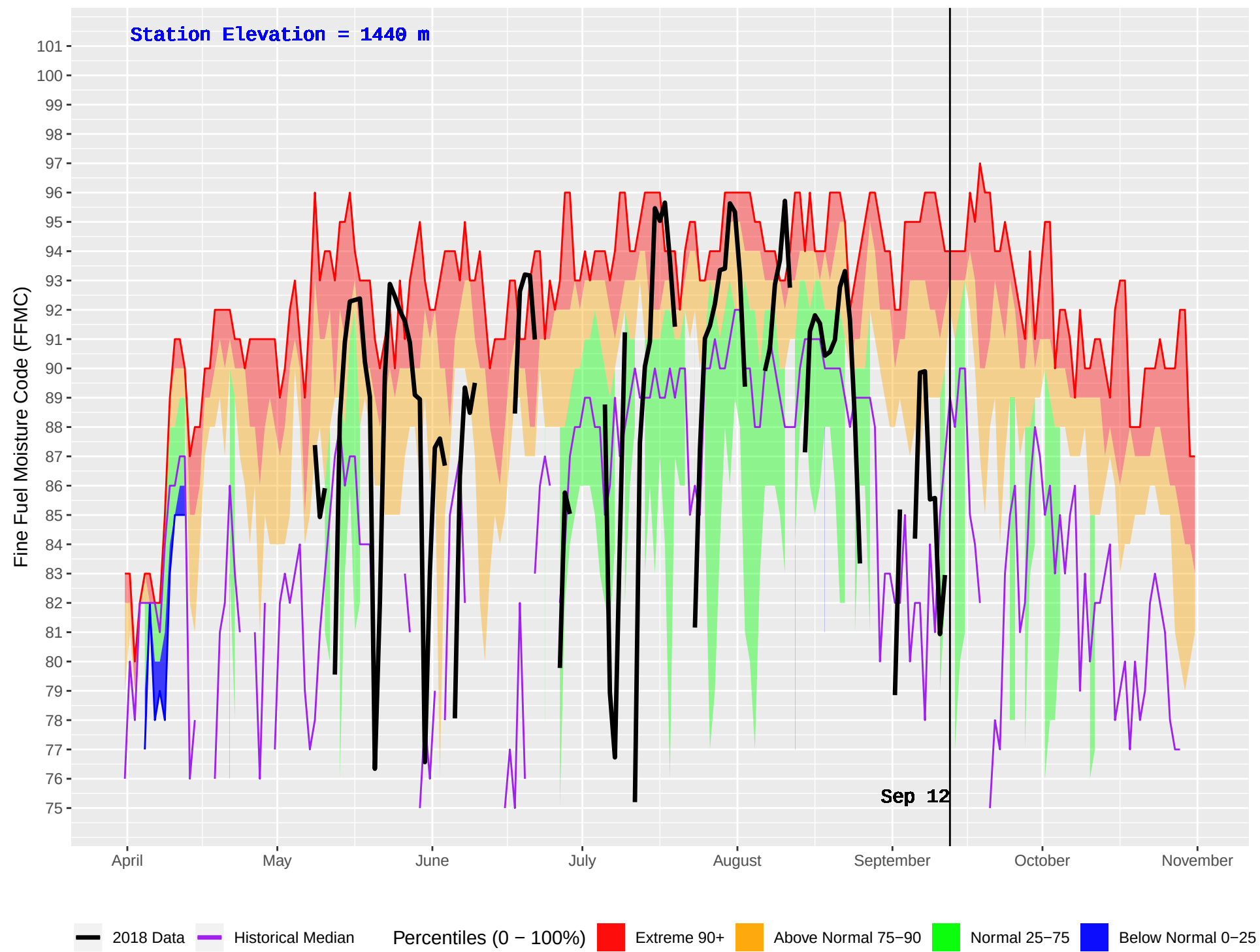
PASKA LAKE (326) : Historical (1999–2016) and Current (2018) Daily Fine Fuel Moisture Code (FFMC)
