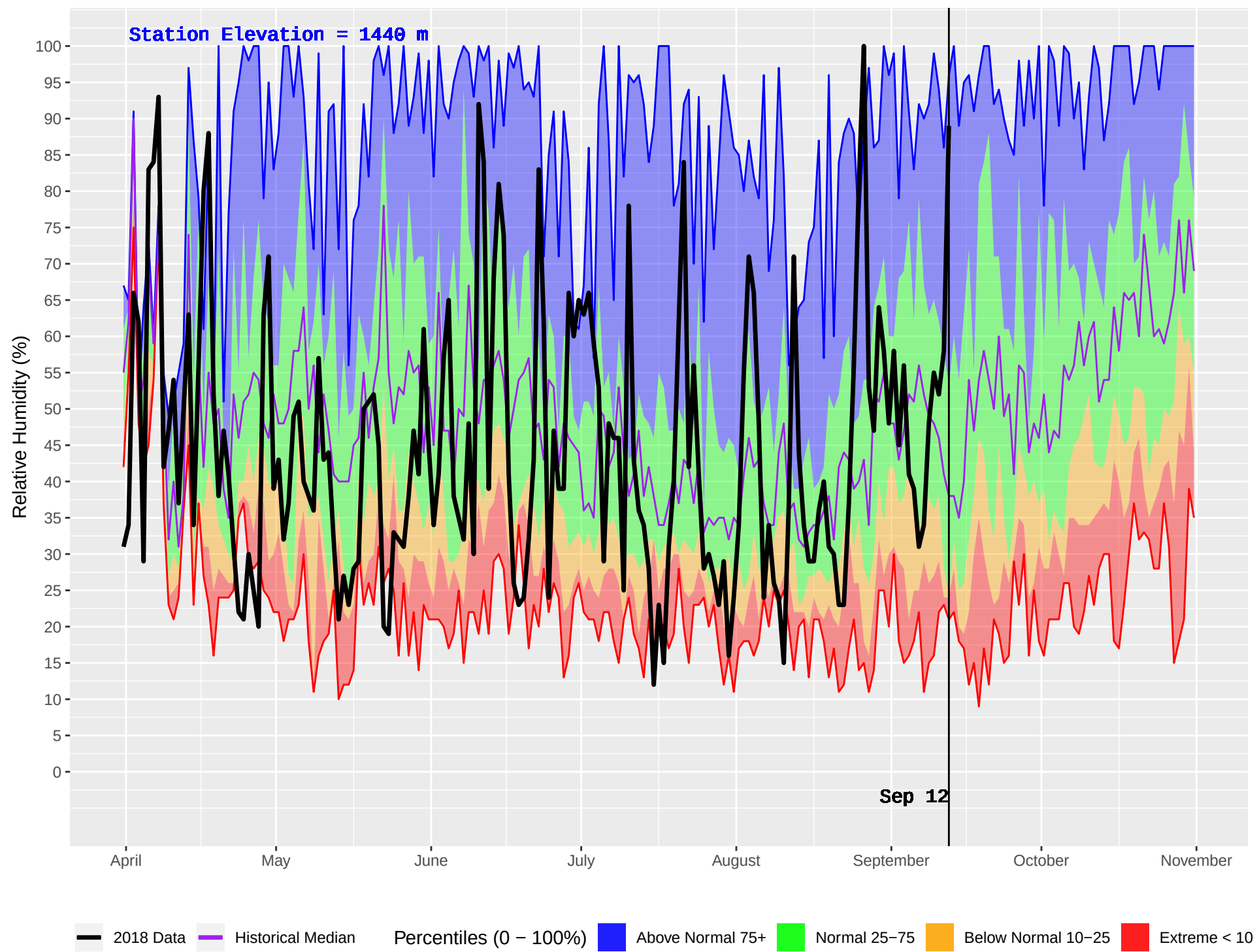
PASKA LAKE (326) : Historical (1999–2016) and Current (2018) Daily Relative Humidity
