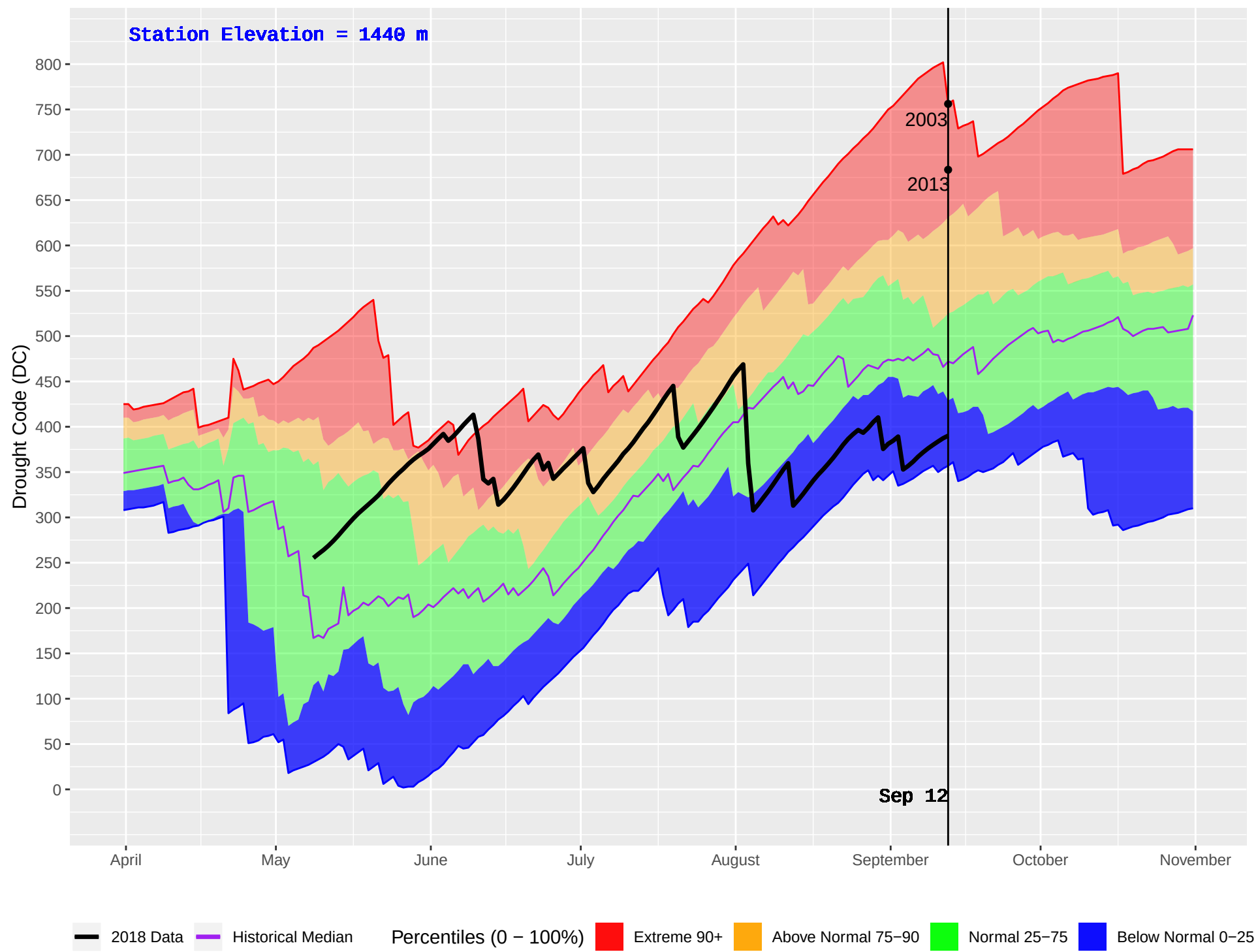
PASKA LAKE (326) : Historical (1999–2016) and Current (2018) Daily Drought Code (DC)
