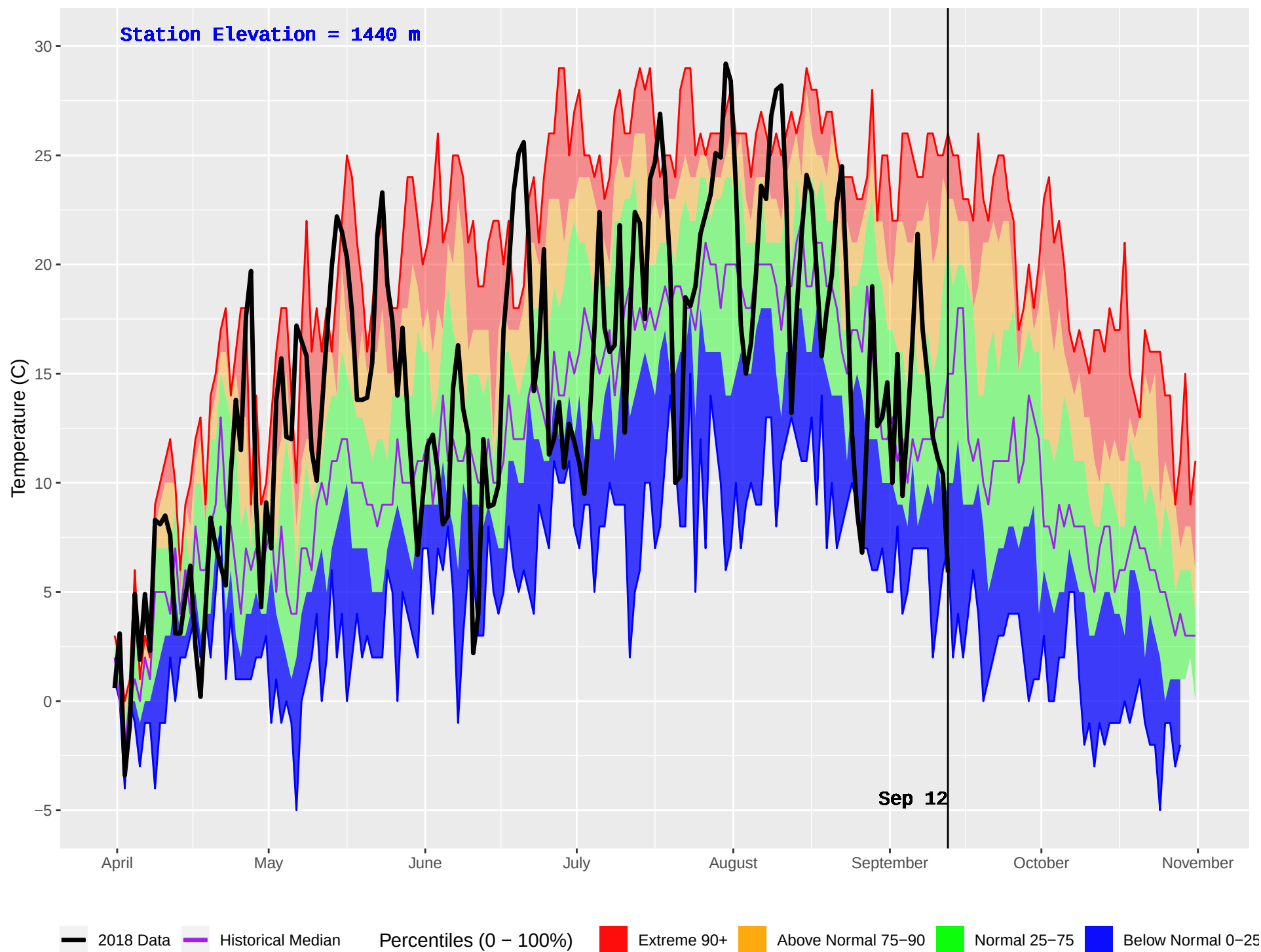
PASKA LAKE (326) : Historical (1999–2016) and Current (2018) Daily Temperature
