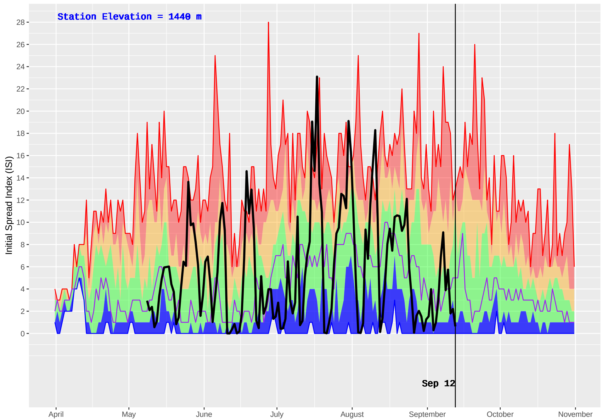
PASKA LAKE (326) : Historical (1999–2016) and Current (2018) Daily Initial Spread Index (ISI)
