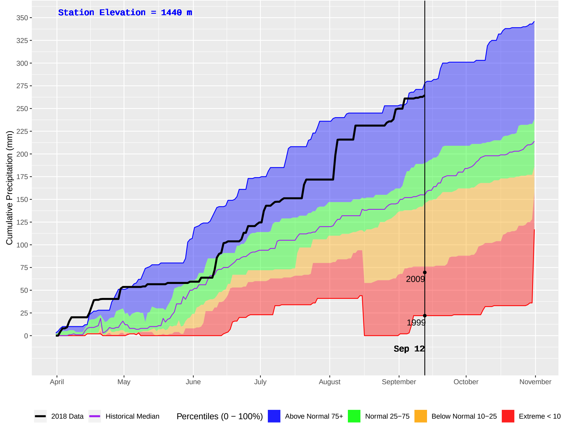
PASKA LAKE (326) : Historical (1999–2016) and Current (2018) Daily Cumulative Precipitation
